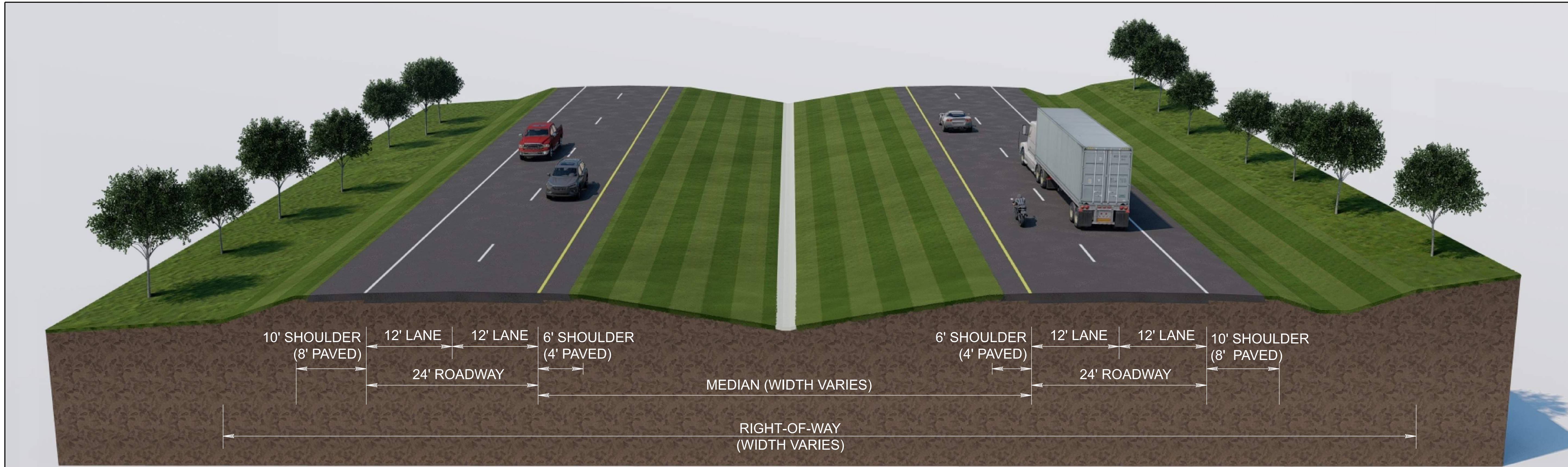
TYPICAL SECTION STATE ROUTE 167 ALTERNATIVE A: FOUR LANE RURAL
