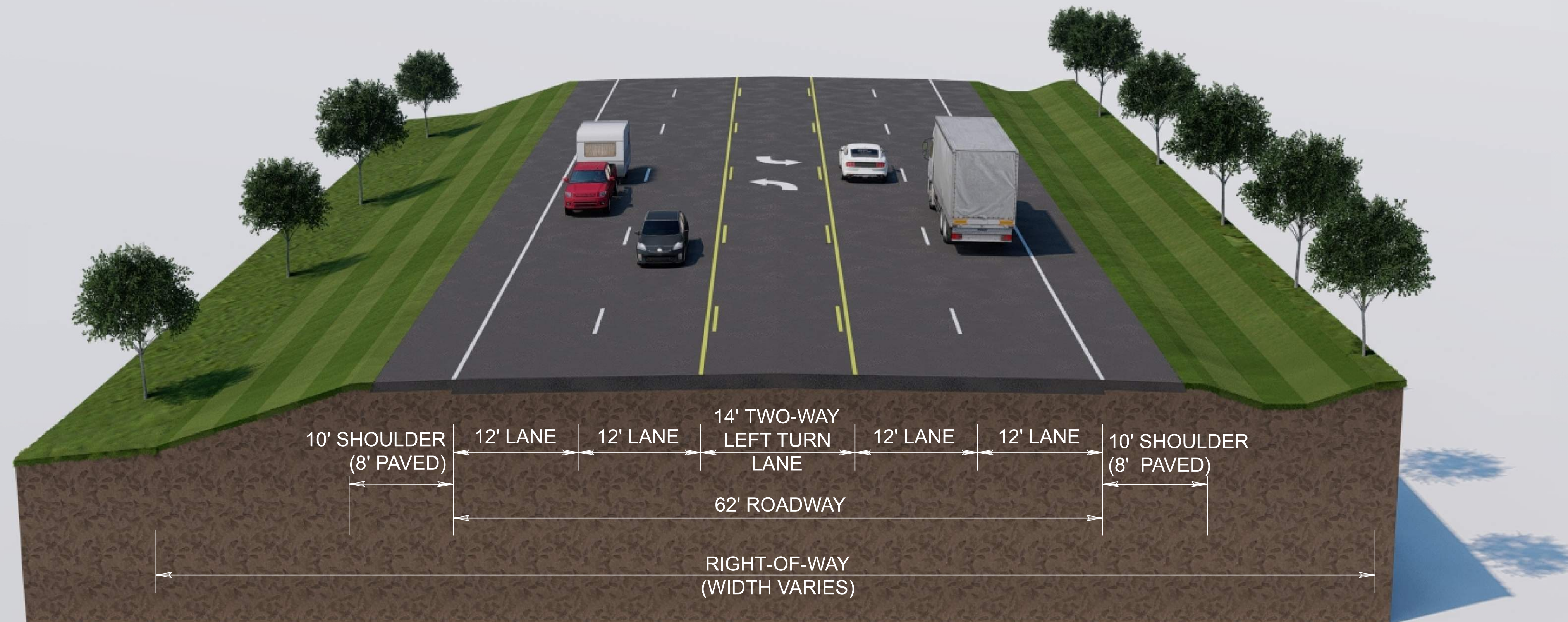
TYPICAL SECTION STATE ROUTE 167 ALTERNATIVE A: FIVE LANE URBAN
