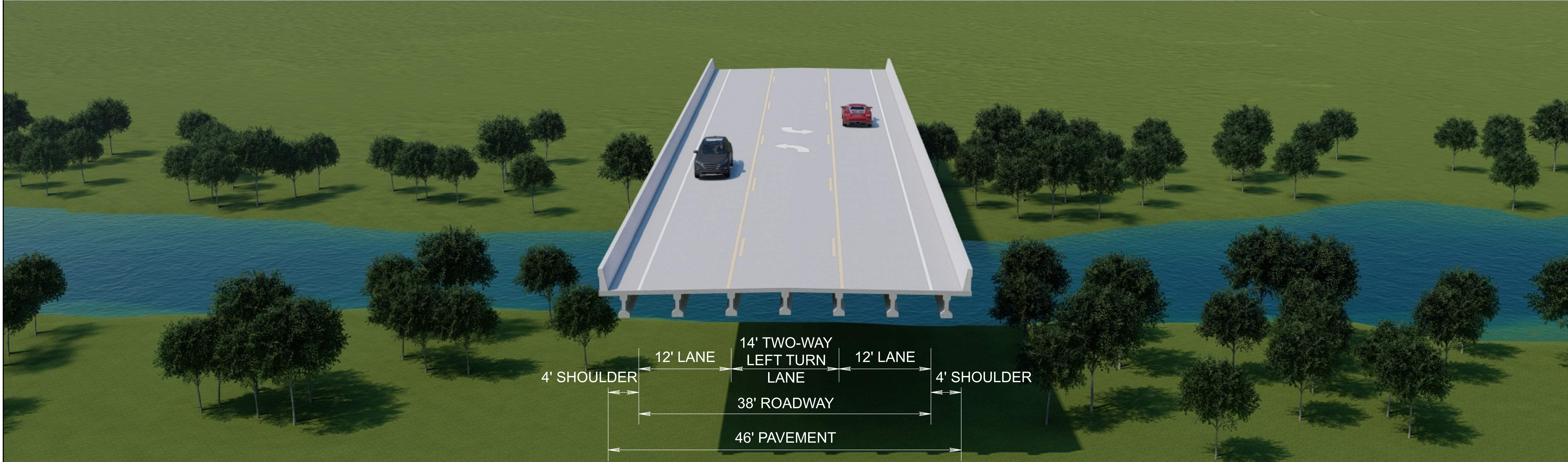
TYPICAL SECTION STATE ROUTE 167 ALTERNATIVE B: THREE LANE BRIDGE
