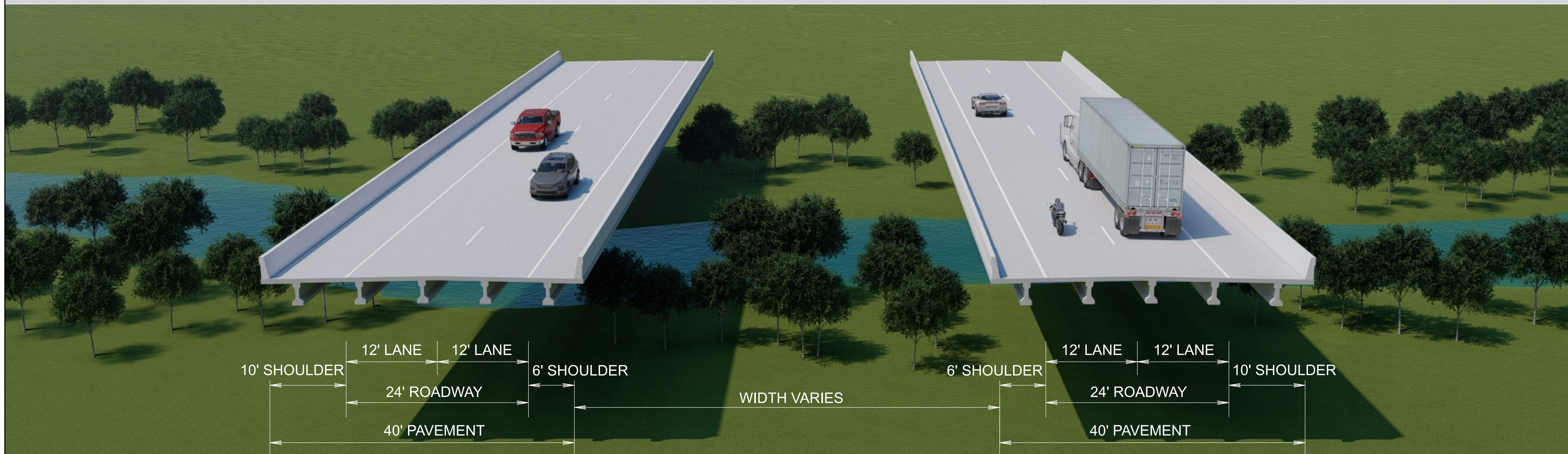
TYPICAL SECTION STATE ROUTE 167 ALTERNATIVE A: FOUR LANE BRIDGE
