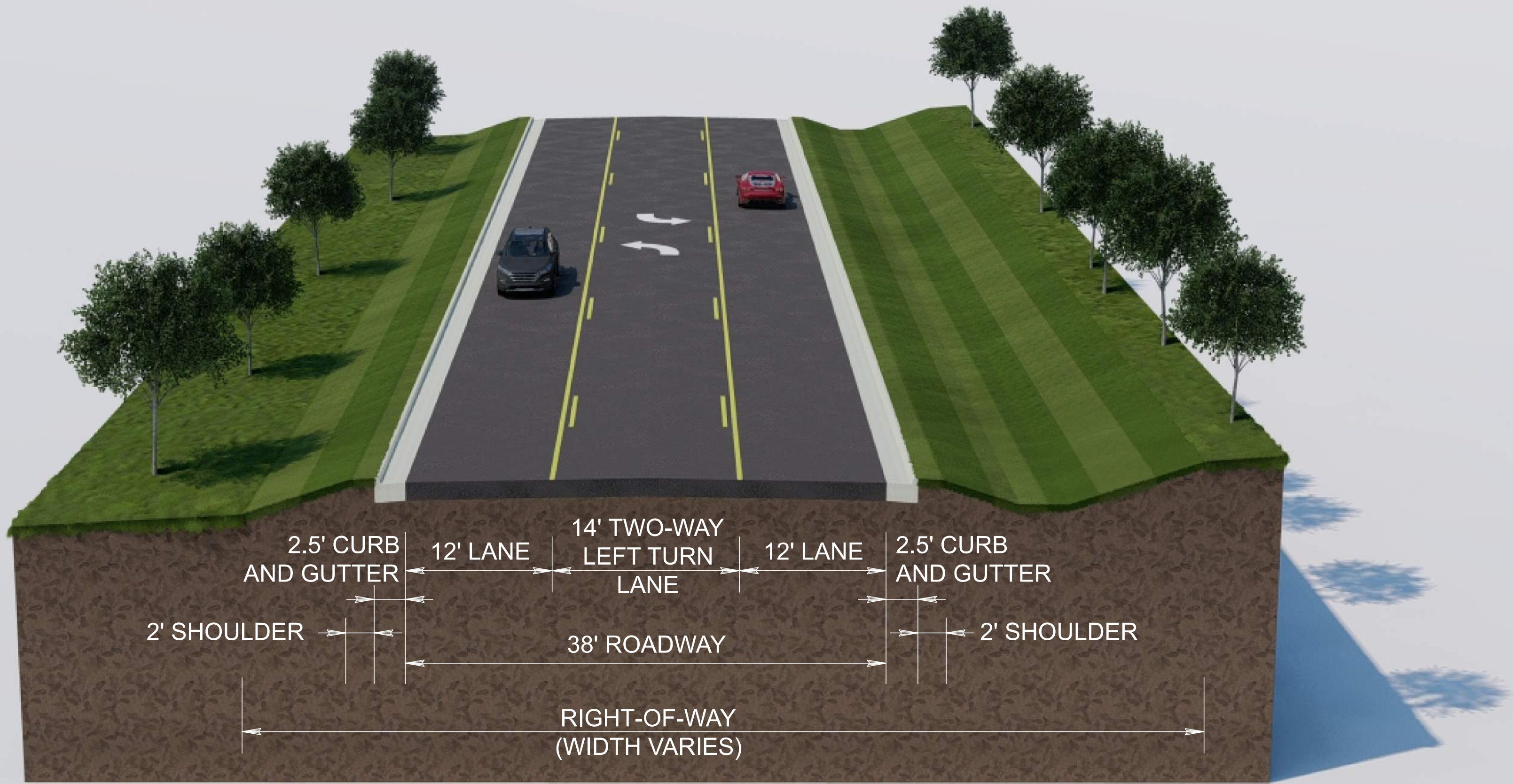
TYPICAL SECTION STATE ROUTE 167 ALTERNATIVE B: THREE LANE URBAN
