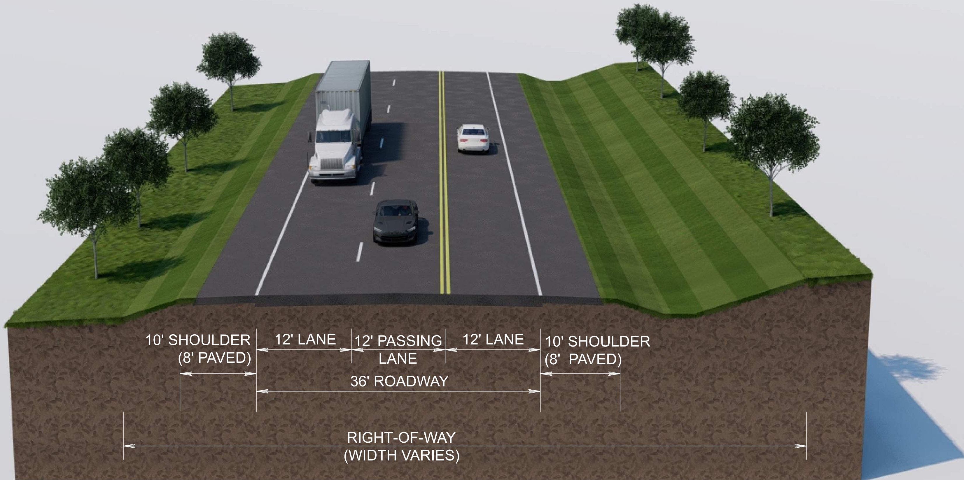
TYPICAL SECTION STATE ROUTE 167 ALTERNATIVE B: ADD PASSING LANE - SOUTHBOUND
