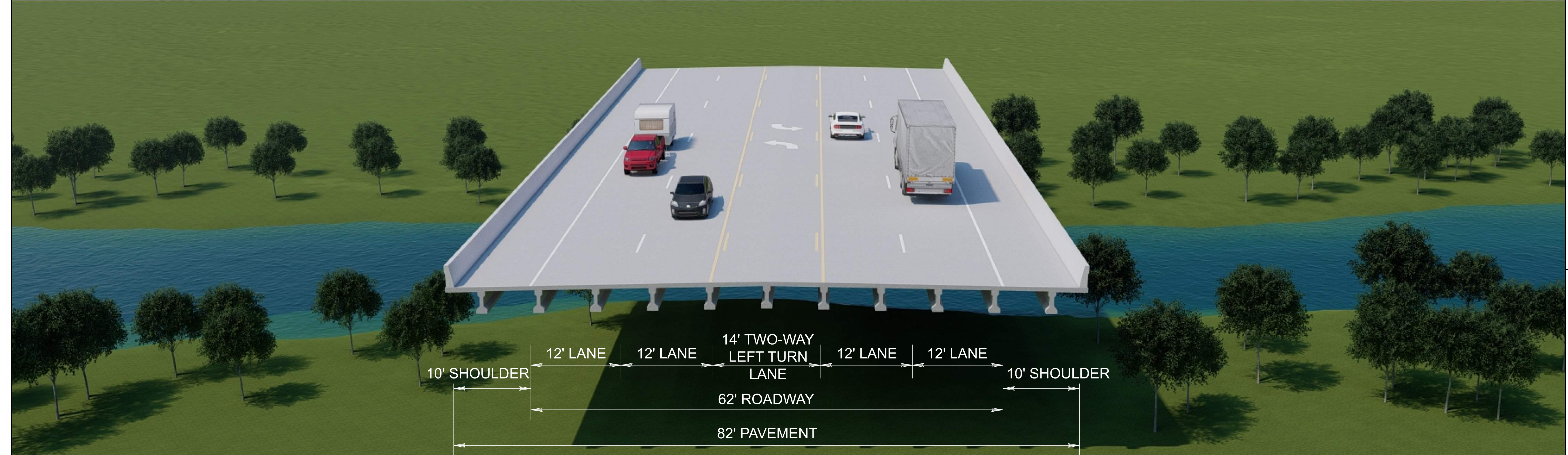
TYPICAL SECTION STATE ROUTE 167 ALTERNATIVE A: FIVE LANE BRIDGE
